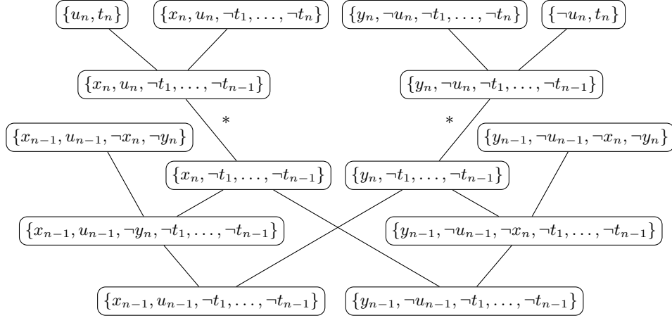
Fig. 3. Portion of a linear size \text{Q}(\mathcal{D}^{\text{rfs}}) -Res refutation of \Psi(n) . The \forall -reduction steps marked with * are forbidden in Q-Res, but are allowed in \text{Q}(\mathcal{D}^{\text{rfs}}) -Res due to Prop. 8.
